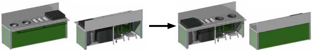
Code 859260 Without door - Access to collectors from the rear
