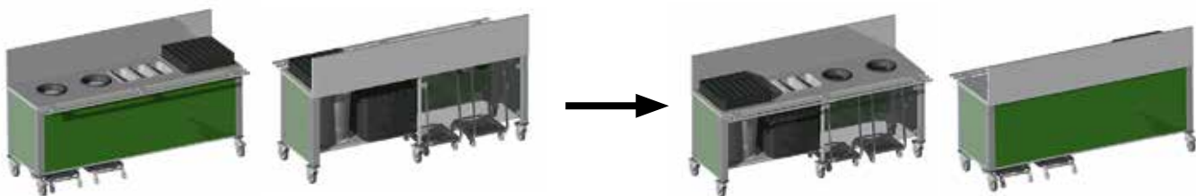
Code 858332 With doors - Access to collectors from the rear
